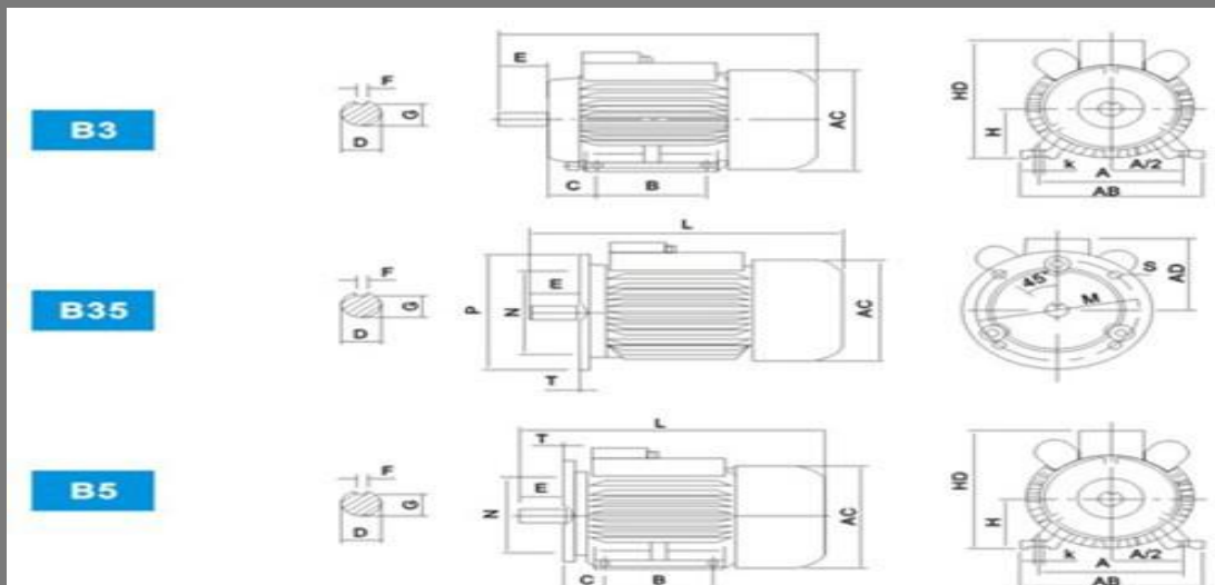
YL SINGLE PHASE MOTOR DIMENSIONS(mm)
